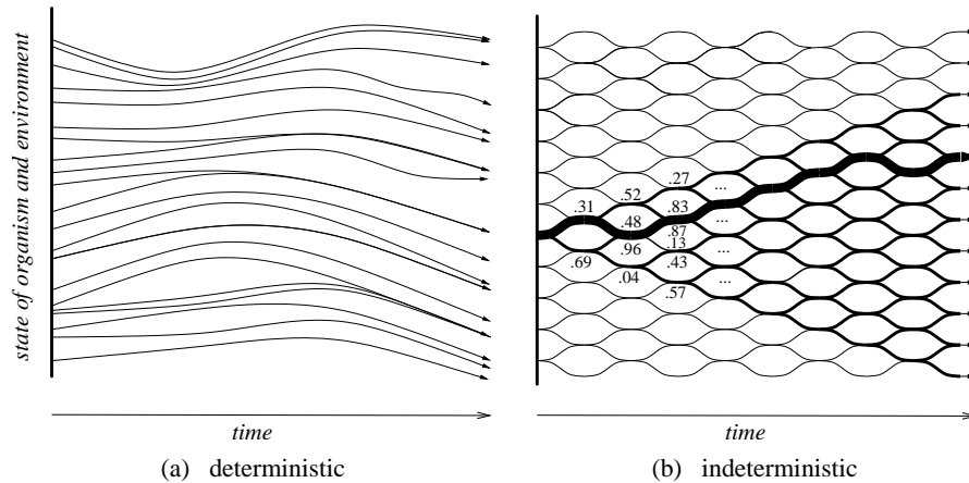
Idealized representations of organism-environment history spaces assuming that biological processes are deterministic (a) or indeterministic (b). Only one dimension of variation in states at a time is represented, and only two-way branching is represented in (b) (where histories beginning from one initial state are highlighted, one history is further emphasized, and probabilities of some branches are indicated).
