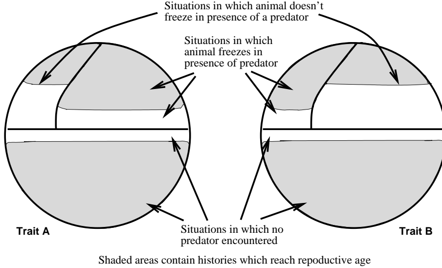
Figure 2. Type A is fitter: A's perform a functional behavior with greater probability. Each point represents an entire history; roughly speaking, the time axis is perpendicular to the page.
